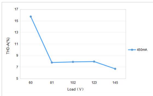
THD Curve
