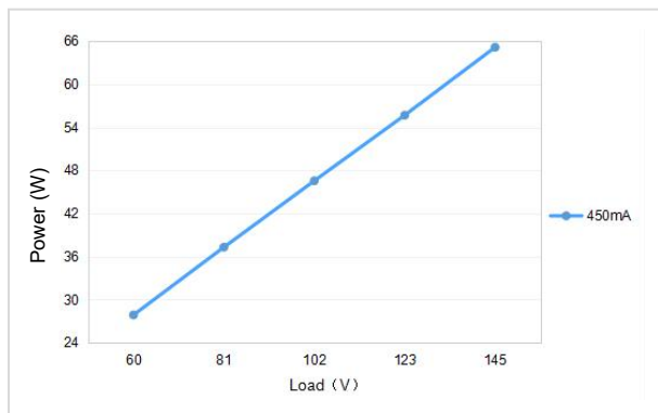
Power Curve
